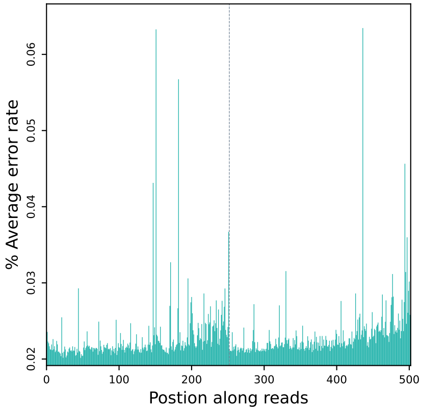
Error rate distribution along reads (R10419)
